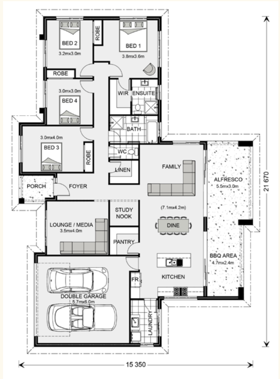
Stillwater (Estate) 235 Classic facade floorplan
