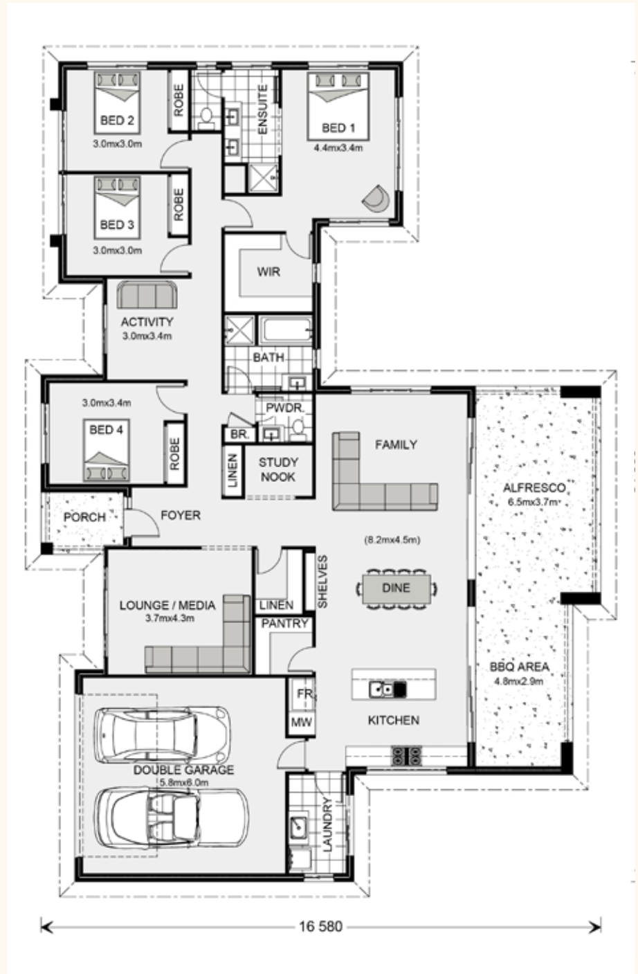
Stillwater (Estate) 285 Classic facade floorplan
