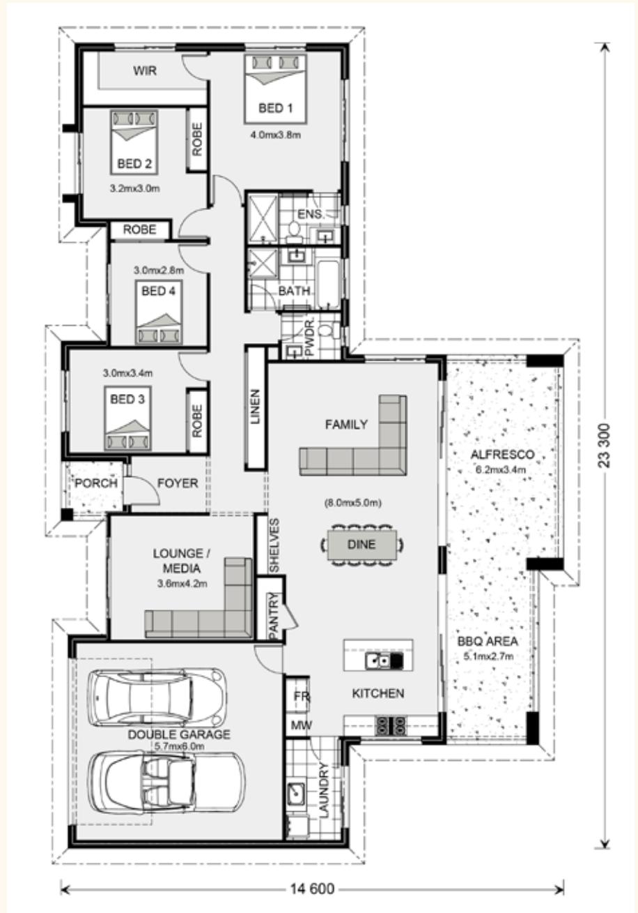
Stillwater (Estate) 250 Classic facade floorplan
